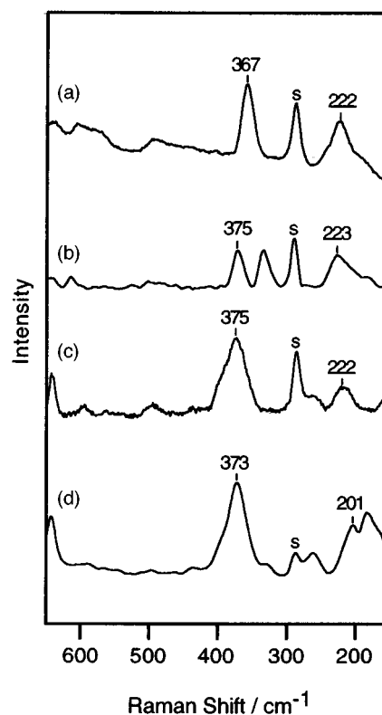
Fig. 1 Low-frequency RR spectra of the deoxy complexes 1 (a), 2 (b), 3 (c) and 4 (d) in \text{CH}_2\text{Cl}_2 with 457.9 nm excitation. Laser power, 60 mW; accumulation time, 60 s; three scans; sample concentration, 1 \text{ mmol dm}^{-3} ; s denotes solvent bands
